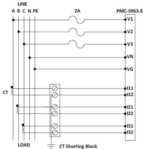
3P4W with 3CTs and no PTs
