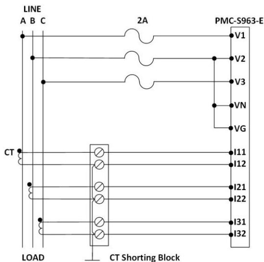
3P3W with 3CTs
