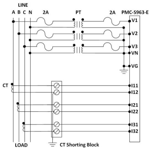
3P4W with 3CTs and 3PTs
